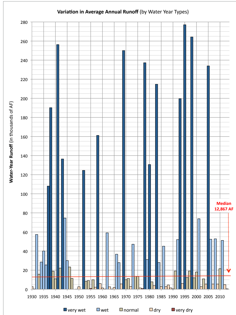
Figure 3.4.2.3.2 Variation in Average Annual Runoff (by Water Year Types). Average annual runoff from each water year year between 1930–2013 (as measured at Foster Park) was used to assign one of five water year categories—very wet, wet, normal, dry, and very dry—to each year. Half of the years are above the median and half below. See “4.4 Appendices” for the “Table of Water Year Types Based on Annual Average Runoff,” for the list of years by water year type, and an explanation of the category divisions.
