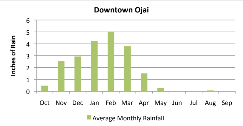
Figure 3.4.2.3.1 Average Monthly Rainfall, Ojai
